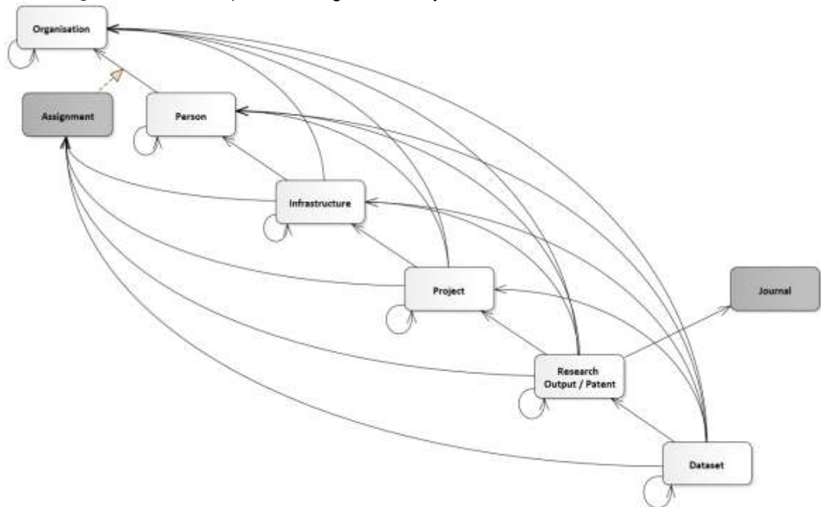
Figure 3: Entity relations
