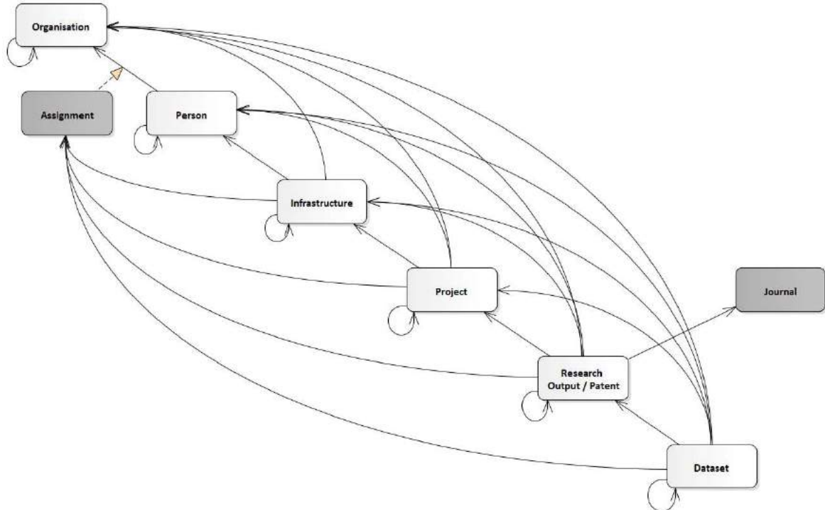
Figure 3: Entity relations
