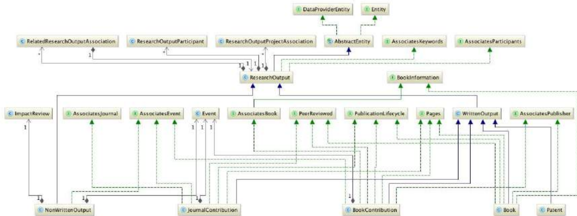
Figure 14 UML class diagram of FRIS research output model classes
