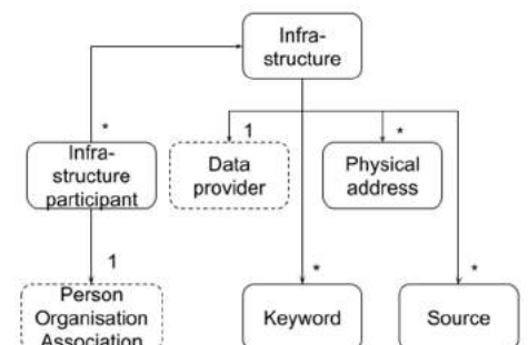
Figure 6: High-level infrastructure model
