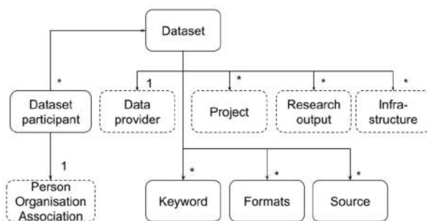
Figure 9: High-level dataset model
