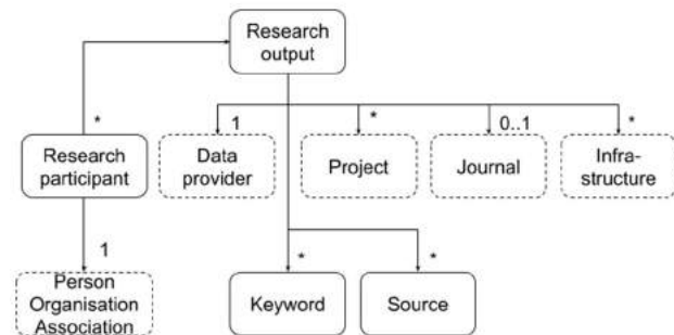
Figure 8: High-level research output model
