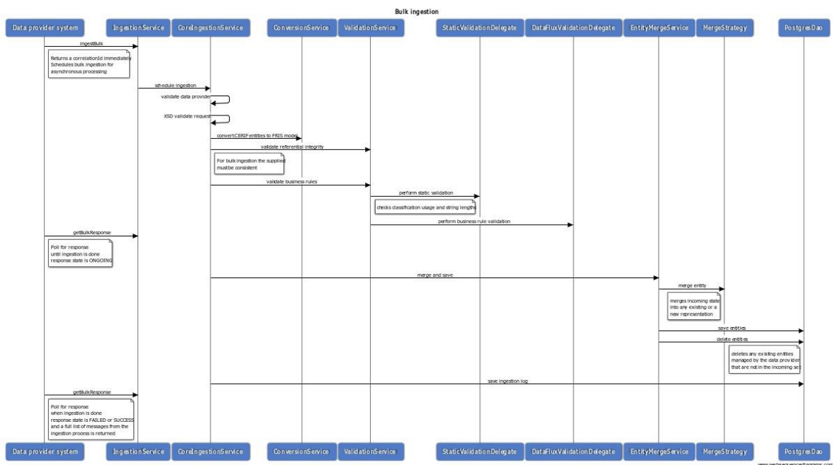
Figure 13 Bulk ingestion sequence diagram
