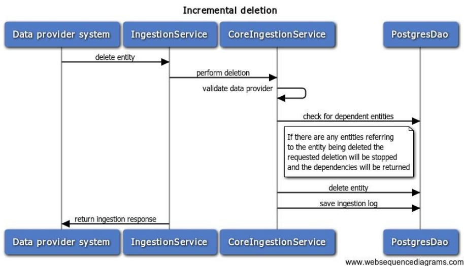
Figure 15 Incremental deletion sequence
