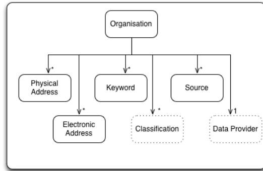
Figure 5 Contents of high-level organisation concept
