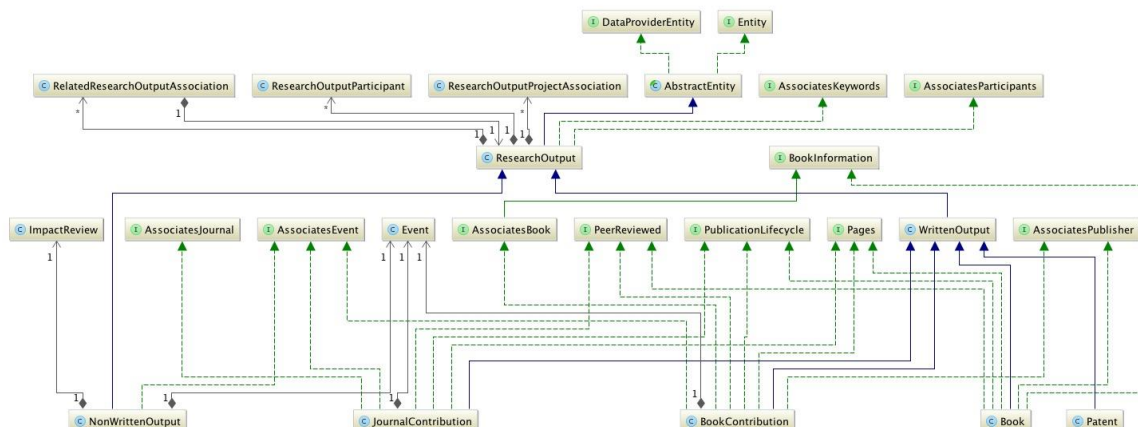
Figure 17 UML class diagram of FRIS research output model classes
