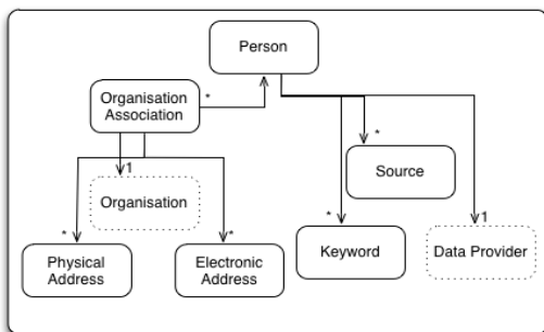
Figure 6 Contents of high-level person concept
