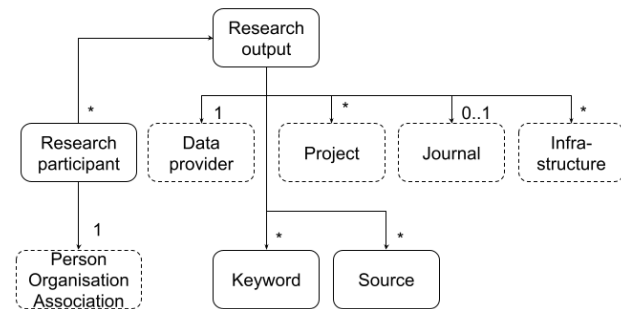
Figure 10: High-level research output model
