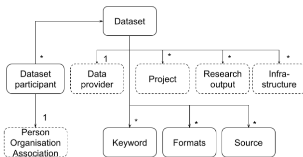
Figure 12: High-level dataset model
