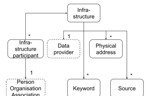
Figure 7: High-level infrastructure model
